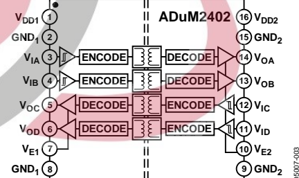
Figure 3. ADuM2402
